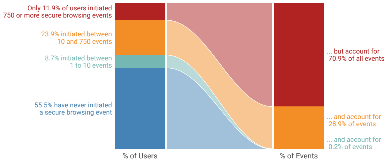
FIGURE 12: DISTRIBUTION OF SECURE BROWSING EVENTS PER USER
