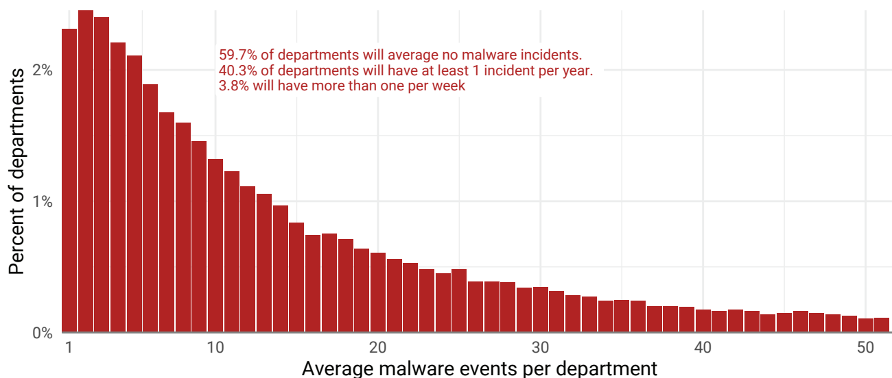
FIGURE 10: AVERAGE MALWARE EVENTS PER DEPARTMENT PER YEAR
